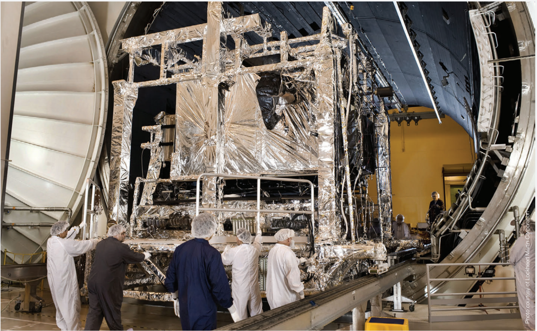
Technicians move equipment into an environmental testing space chamber at Lockheed Martin.
